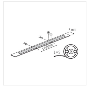
LCOB 3W/M 24 IP00-CW
