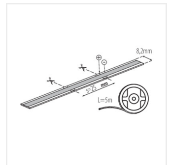
LCOB 3W/M 24 IP65-EW
