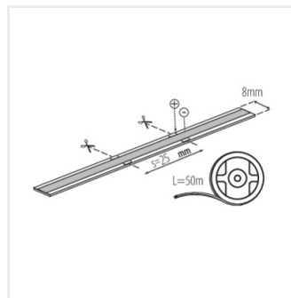
LCOBC 3W/M 24 IP00-EW
