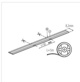
LCOB 10W/M 24 IP65-EW
