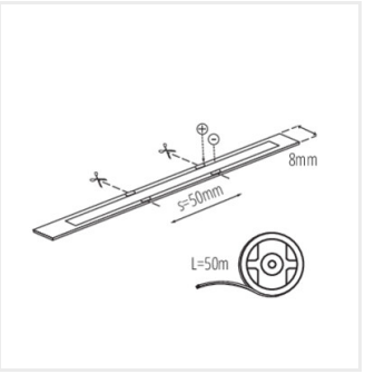
LCOBC 10W/M 24IP00-CW
