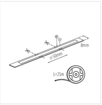
LCOBB 10W/M 24IP00-CW
