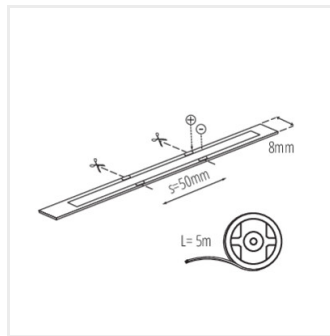
LCOB 10W/M 24 IP00-WW
