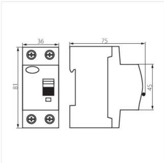
KRD6-2/25/30
