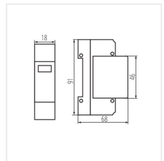
KSPD-T1T2 275/50 1P
