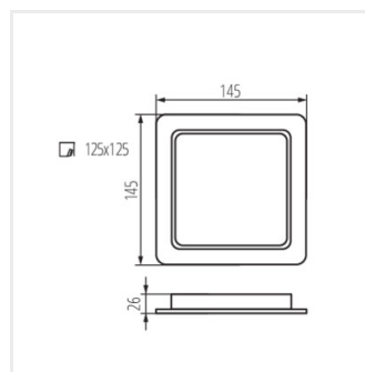
TAVO LED DL 12W CCT
