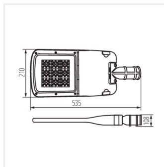
PRO-S S 50W-ZH NW Data of issue: 06.03.2023, 10:05
