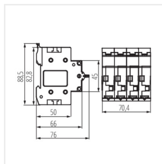
KCS-40A/4P
