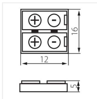
CONNECTOR 8
