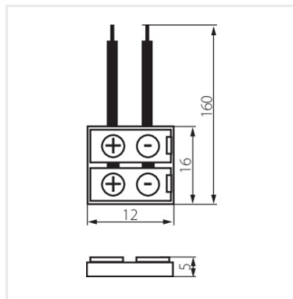
CONNECTOR 8-CP
