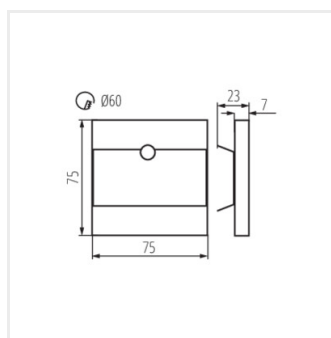
TERRA LED PIR B
