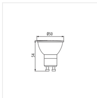
GU10 2,7W-WW LED
