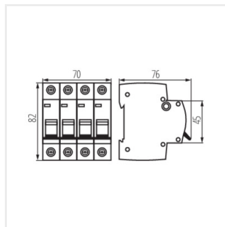
KMB6-B25/4
