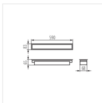
ALD-SH-WW-MAT-W-PT
