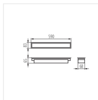
ALD-SH-WW-MPR-W-PT
