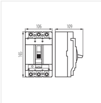
KMCCB-F-200A
