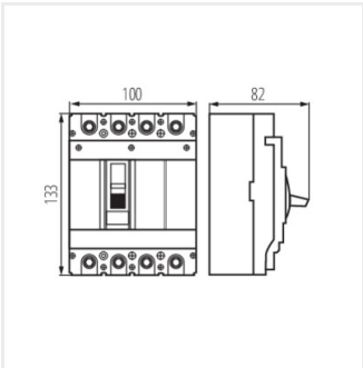
KMCCB-F-125A-4P
