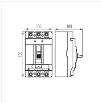
KMCCB-F-250A
