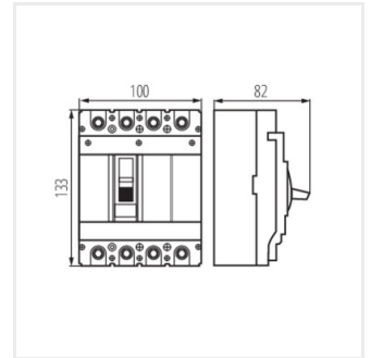
KMCCB-F-125A-4P
