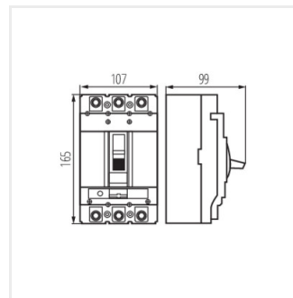
KMCCB-RT-250A
