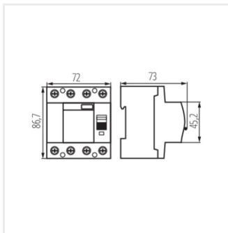
KRD10-4/63/300-B
