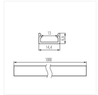
PROFILO J SET-MI-AL
