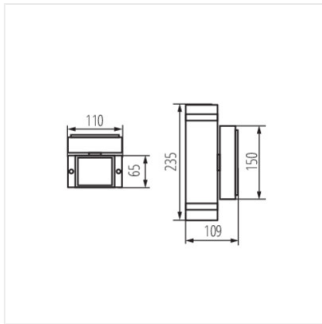
ZEW EL-235J
