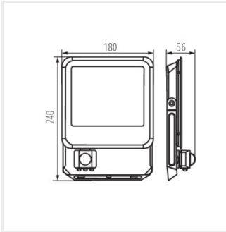
IQ-LED FL-50W-NW-SE
