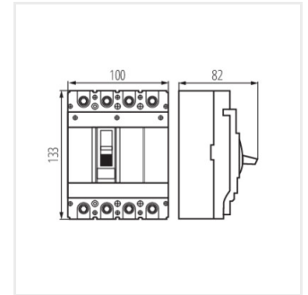
KMCCB-F-125A-4P
