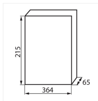
DB118F 1X18P/FMD
