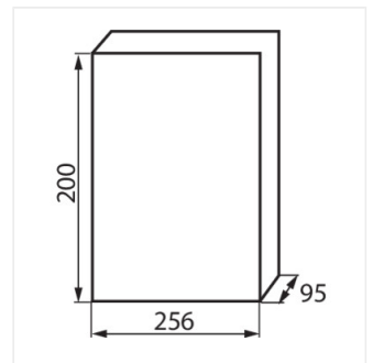
DB112S 1X12P/SMD
