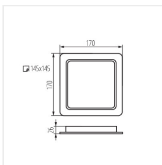
TAVO LED DL 18W CCT
