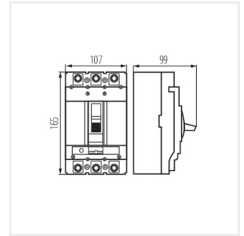
KMCCB-RT-250A
