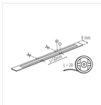
LCOBL 7,5W/M24IP00-CW
