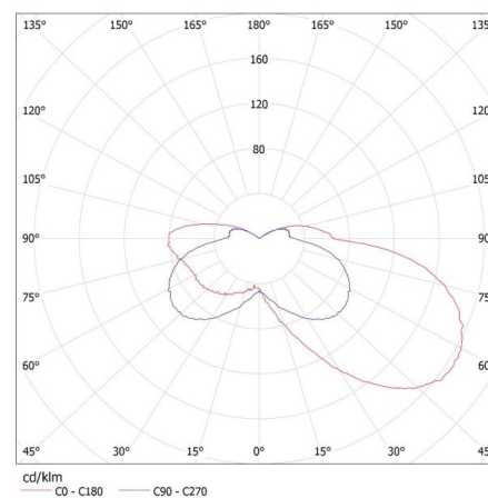
KANLUX S.A. (kat 23108) SABIK LED WW / LDC (Polar) Luminaire: KANLUX S.A. (kat 23108) SABIK LED WW Lamps: 1 x SABIK LED WW
