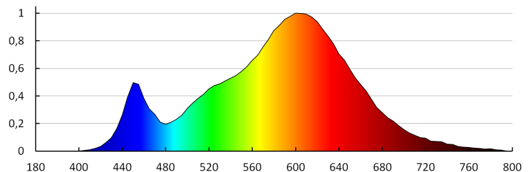
KANLUX S.A. (kat 23108) SABIK LED WW / LDC (Polar) Luminaire: KANLUX S.A. (kat 23108) SABIK LED WW Lamps: 1 x SABIK LED WW
