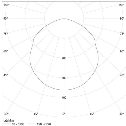
KANLUX S.A. (kat 27155+33193+33196) HB PRO LED HI 100W-NW + LENS 120D + GRID / LDC (Polar)
