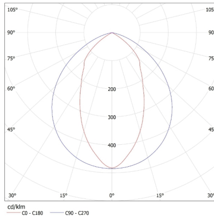
MILEDO (kat 31058) RSTR N 236/4LED/NT i T8 Miledo / LDC (Polar) Luminaire: MILEDO (kat 31058) RSTR N 236/4LED/NT i T8 Miledo Lamps: 2 x T8 LED N 18W-ND
