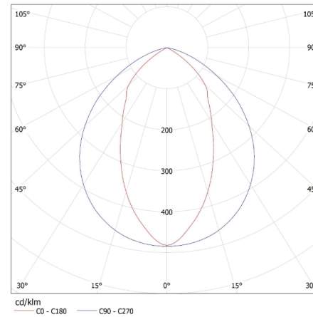
MILED0 (kat 31058) RSTR N 236/4LED/NT i T8 Miledo / LDC (Polar) Luminaire: MILED0 (kat 31058) RSTR N 236/4LED/NT i T8 Miledo Lamps: 2 x T8 LED N 18W-1W
